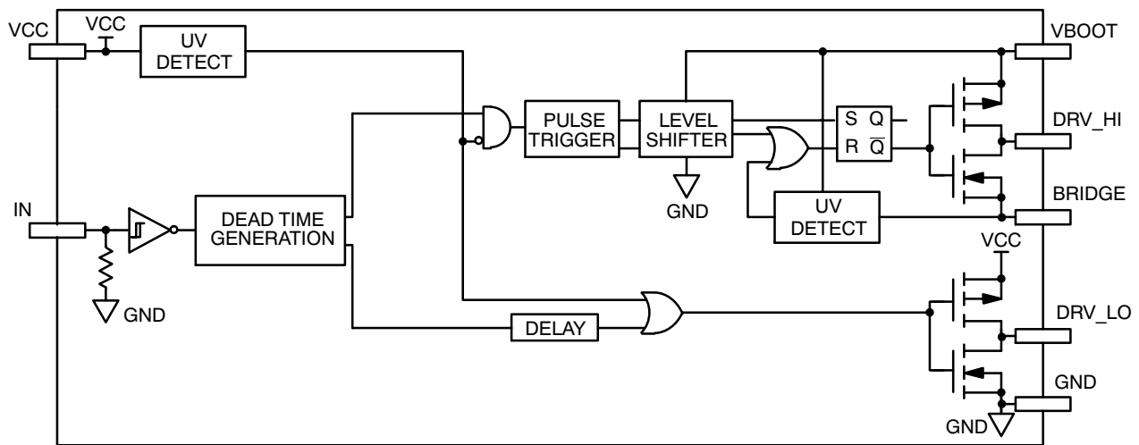
Figure 3. Detailed Block Diagram
