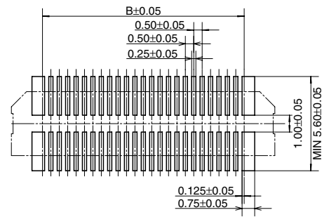
Recommended metal mask pattern
