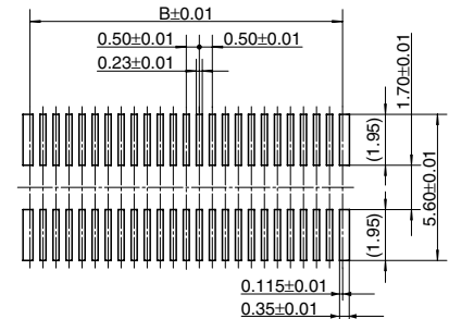
Recommended metal mask pattern Metal mask thickness: Here, 120 \mu\text{m} (Opening area ratio: 78%)
