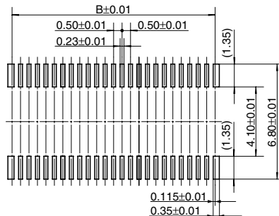
Recommended metal mask pattern Metal mask thickness: Here, 120 \mu\text{m} (Opening area ratio: 69%)
