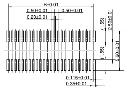
Recommended metal mask pattern Metal mask thickness: Here, 150 \mu\text{m} (Opening area ratio: 62%)
