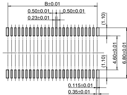
Recommended metal mask pattern Metal mask thickness: Here, 120 \mu\text{m} (Opening area ratio: 69%)
