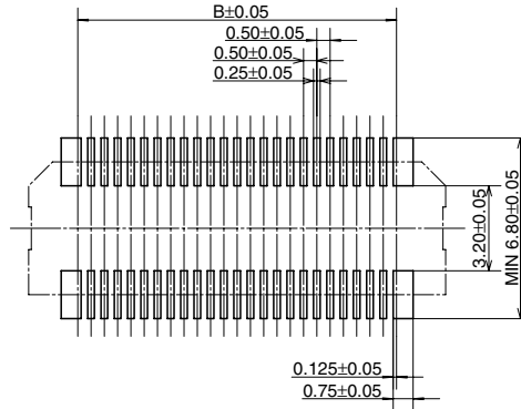
Recommended metal mask pattern Metal mask thickness: Here, 150 \mu\text{m} (Opening area ratio: 56%)
