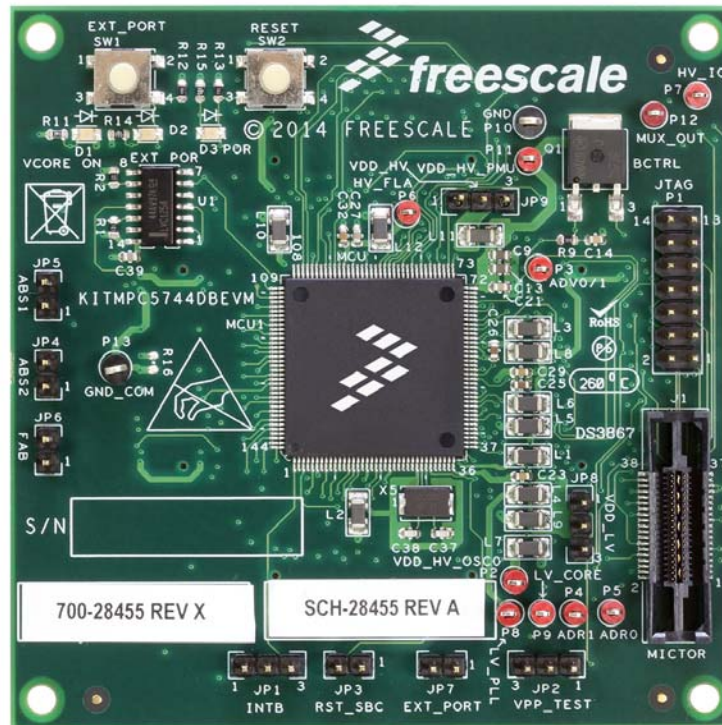
Figure 1. KITMPC5744DBEVM
