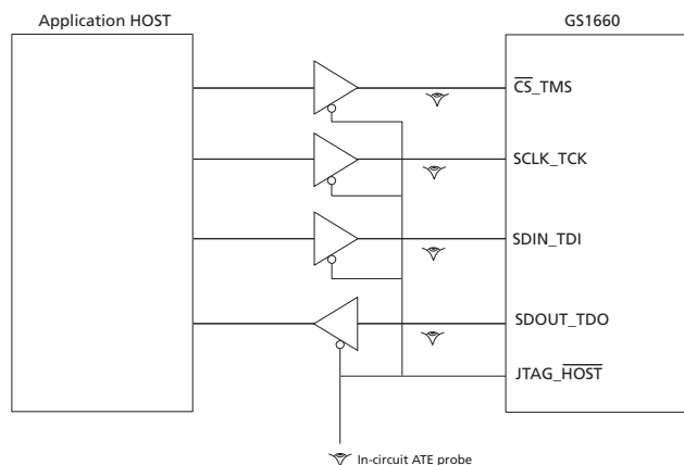
Figure 4-31: In-Circuit JTAG
