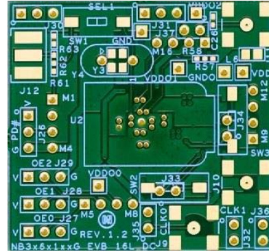
Figure 7. QFN16 Daughter Board Top View
