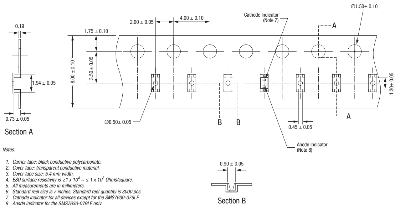
Figure 6. SC-79 Tape and Reel Dimensions
