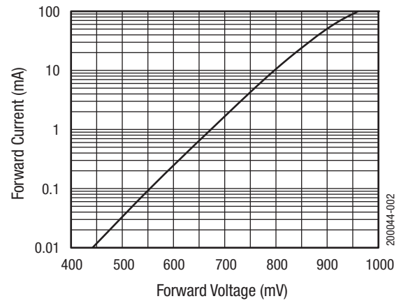
Figure 2. DC Characteristic
