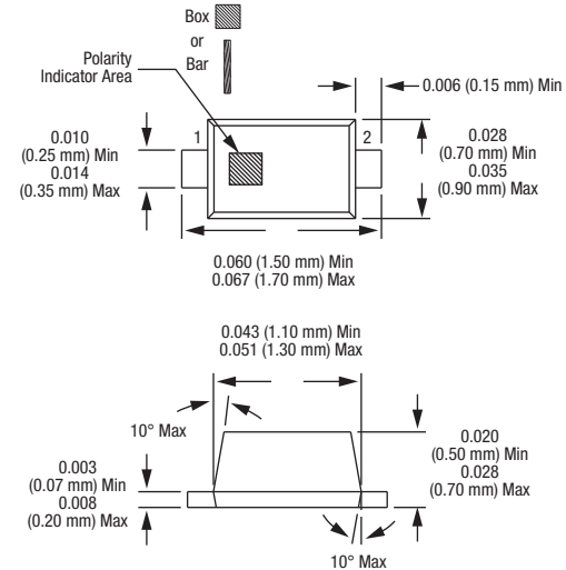
Figure 5. SC-79 Package Dimension Drawing
