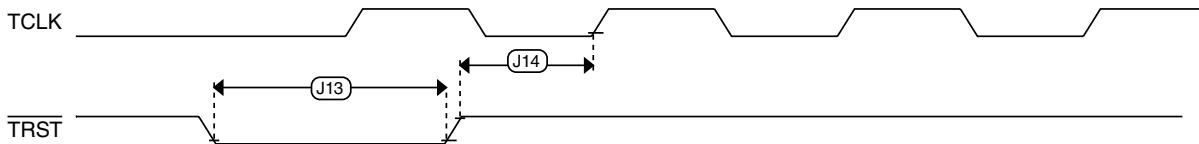
Figure 10. TRST timing
