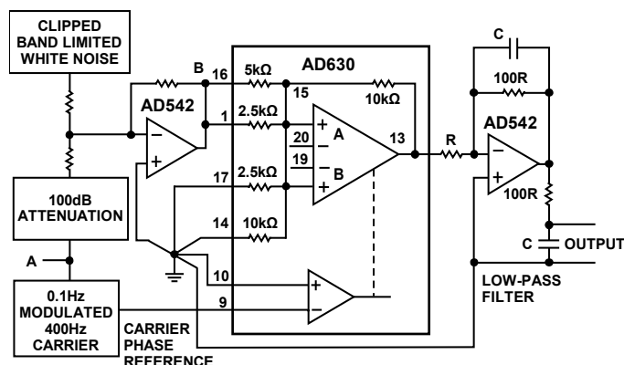
Figure 35. Lock-In Amplifier
