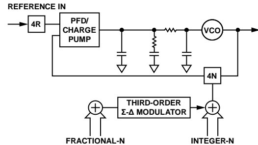
Figure 23. Fractional-N PLL
