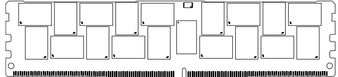
Figure 1: 288-Pin LRDIMM (MO-309, R/C-B, R/C-B1)
