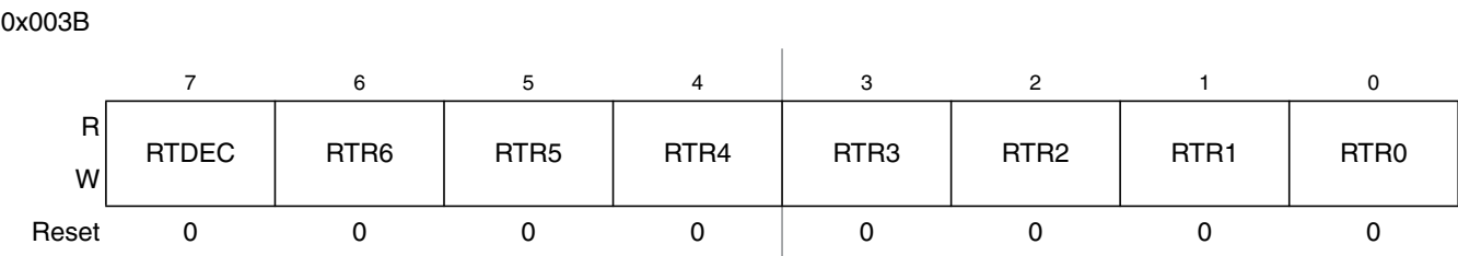
Figure 4-11. S12CPMU_UHV RTI Control Register (CPMURTI)
