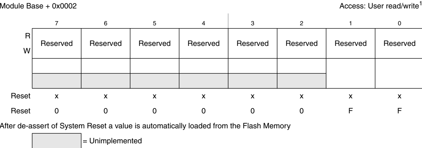
Figure 14-4. Reserved Register
