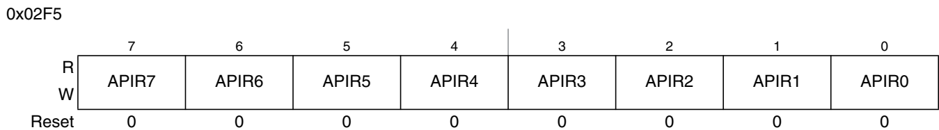
Figure 4-23. Autonomous Periodical Interrupt Rate Low Register (CPMUAPIRL)
