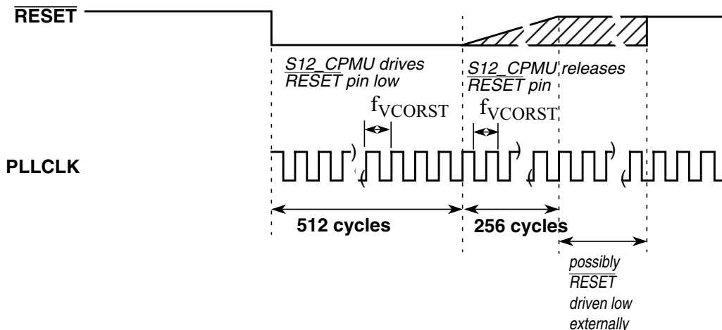
Figure 4-37. RESET Timing
