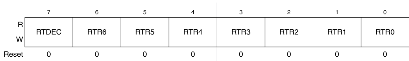
Figure 4-11. S12CPMU_UHV RTI Control Register (CPMURTI)
