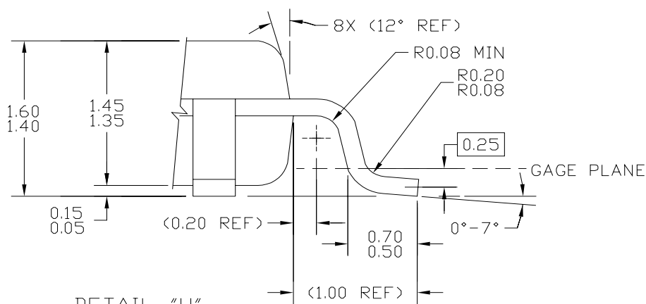
DETAIL "H"
