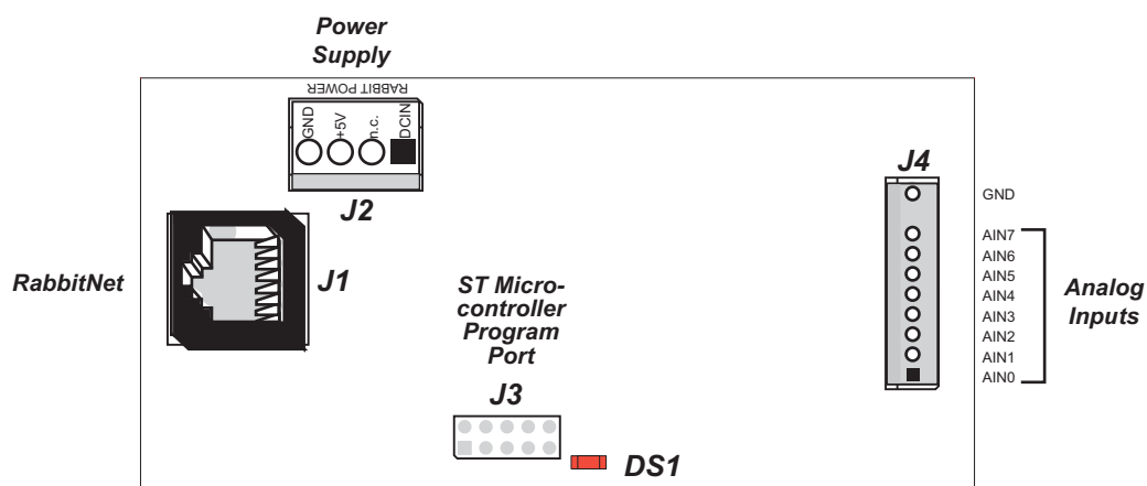
Figure 20. A/D Converter Card Pinouts
