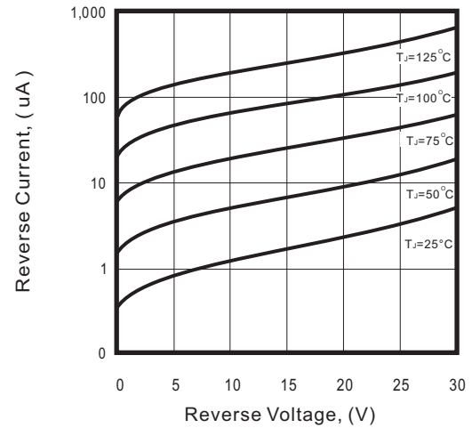
Fig.2 - Reverse Characteristics
