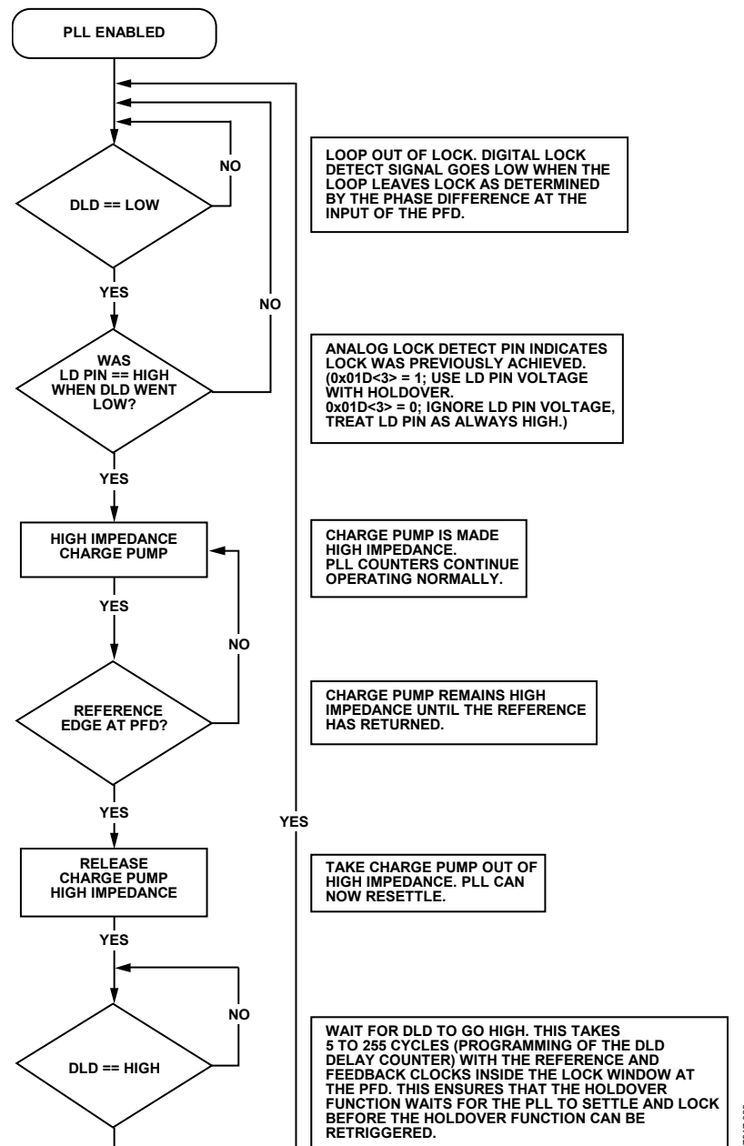
Figure 44. Flowchart of Automatic/Internal Holdover Mode
