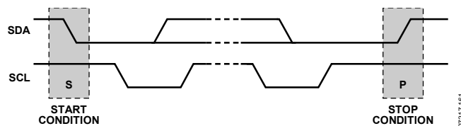
Figure 54. Start and Stop Condition
