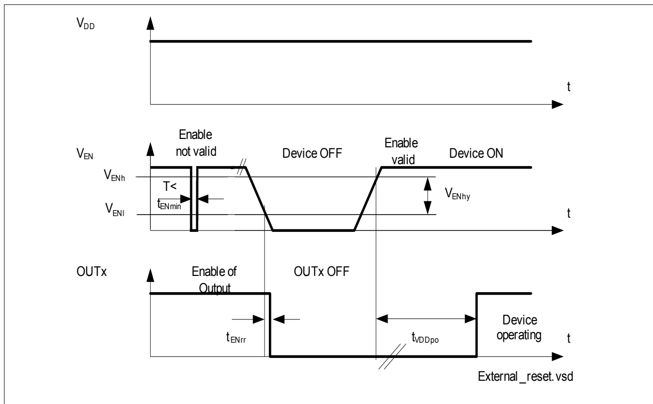
Figure 8 Timing
