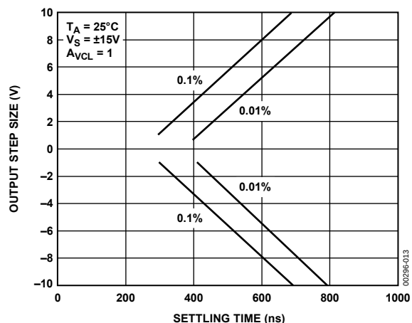
Figure 13. Step Size vs. Settling Time
