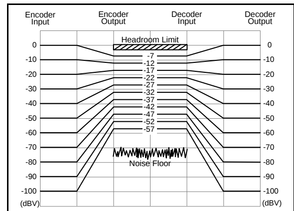
Figure 23. Butterfly diagram of the High-performance 2:1 compander ( f > 1.53\text{kHz} ).
