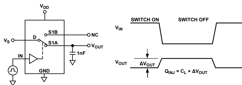
Figure 26. Charge Injection
