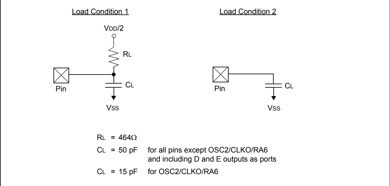
FIGURE 31-3: LOAD CONDITIONS FOR DEVICE TIMING SPECIFICATIONS
