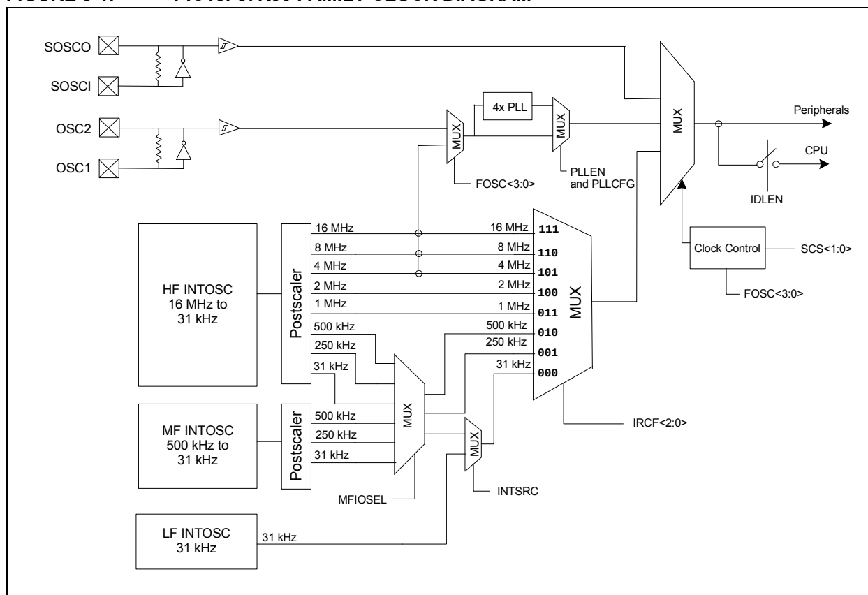
FIGURE 3-1: PIC18F87K90 FAMILY CLOCK DIAGRAM
