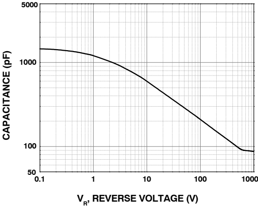
Figure 7. Capacitance vs. Reverse Voltage
