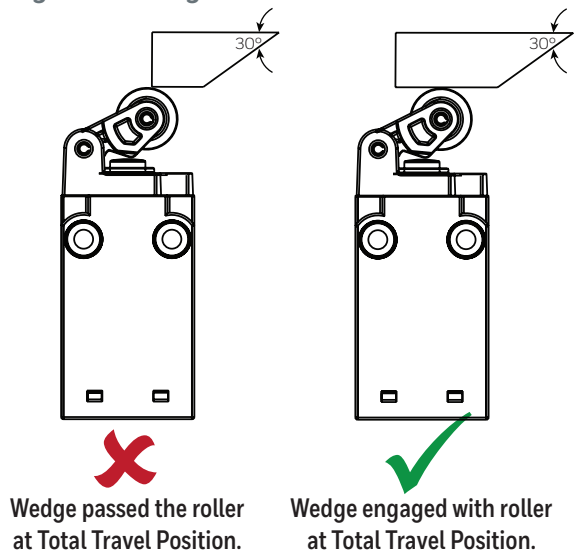
Figure 17. Wedge Actuation
