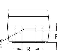
ANODE (+) END VIEW
