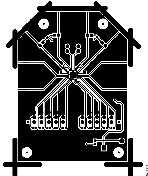
Figure 45. Differential-to-Differential Characterization Board Circuit Side Layout
