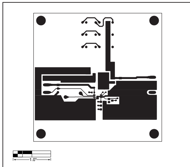
Figure 3. MAX1698 EV Kit PC Board Layout—Component Side
