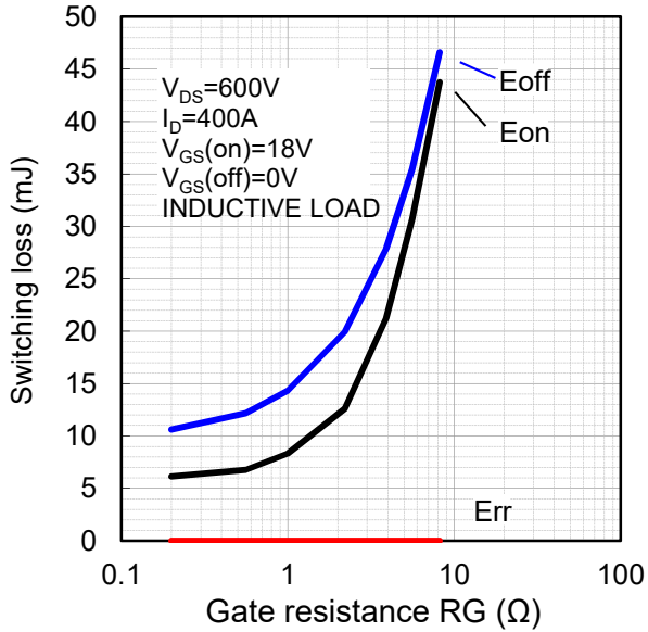
Fig.21 Switching loss vs gate resistance at 25°C (TYP)
