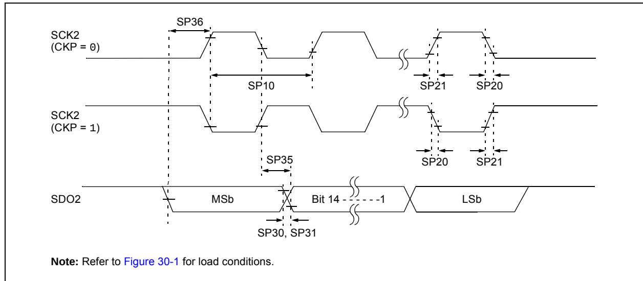
FIGURE 30-13: SPI2 MASTER MODE (HALF-DUPLEX, TRANSMIT ONLY, CKE = 1) TIMING CHARACTERISTICS
