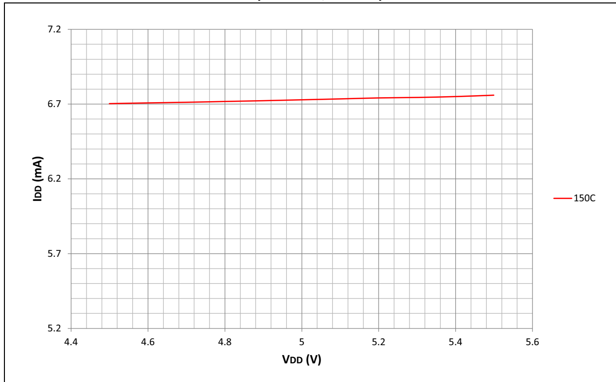
FIGURE 33-2: TYPICAL I DD vs. V DD (EC MODE, 10 MIPS)
