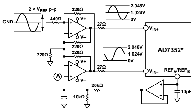
Figure 22. Dual Op Amp Circuit to Convert a Single-Ended Bipolar Signal into a Differential Unipolar Signal
