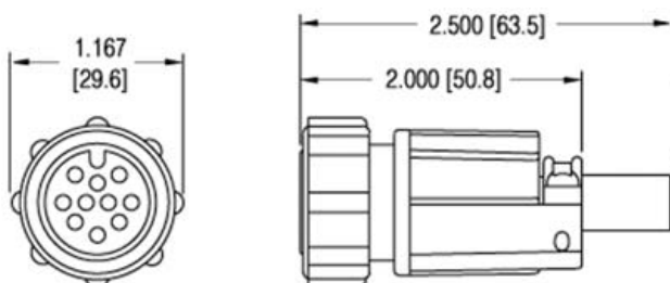
CABLE END CONNECTOR STYLE 3 THREADED BACKSHELL
