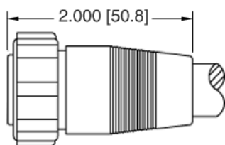
CABLE END ASSEMBLY STRAIGHT BOOT 0.545 [13.8] MAX. CABLE O.D.
