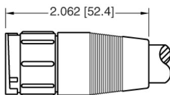
CABLE TO CABLE ASSEMBLY STRAIGHT BOOT 0.545 [13.8] MAX. CABLE O.D.
