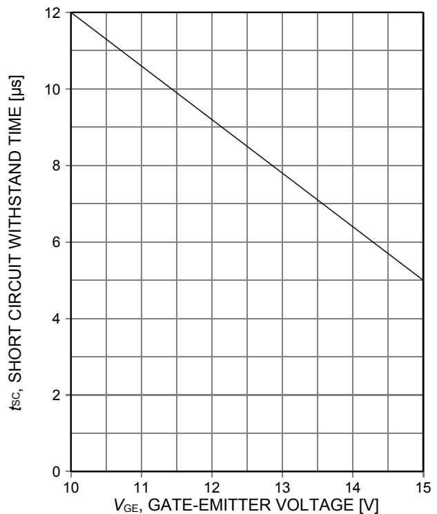
Figure 20. Short circuit withstand time as a function of gate-emitter voltage ( V_{CE}=400V, \text{start at } T_j=25^\circ C, T_{jmax}\leq 150^\circ C )
