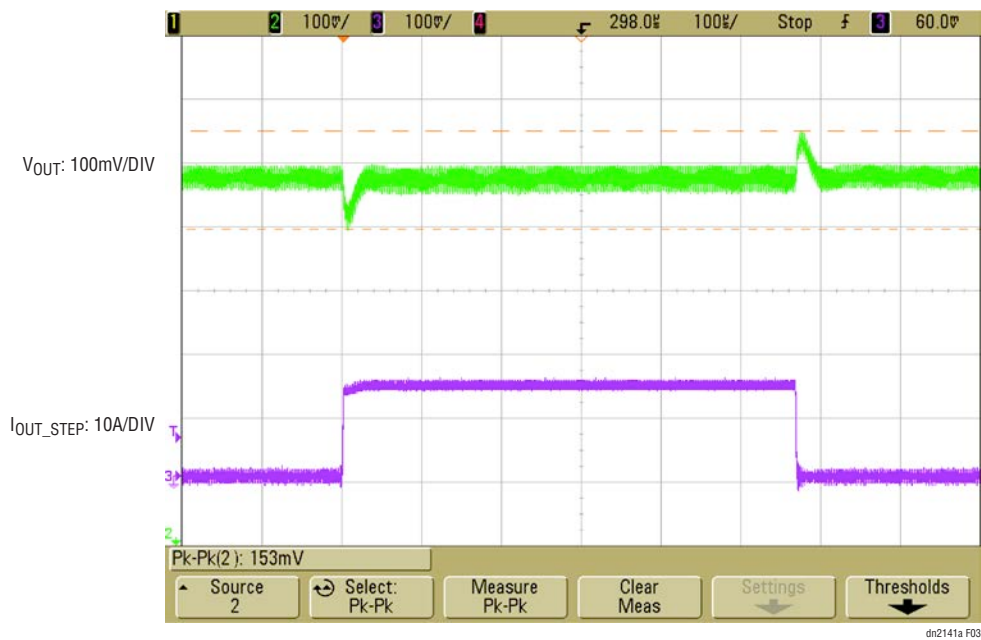
Figure 3. Measured Load Transient, V_{IN} = 12V , V_{OUT1} = 1.0V , I_{STEP} = 5A to 20A
