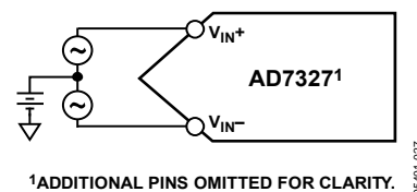
1ADDITIONAL PINS OMITTED FOR CLARITY.
