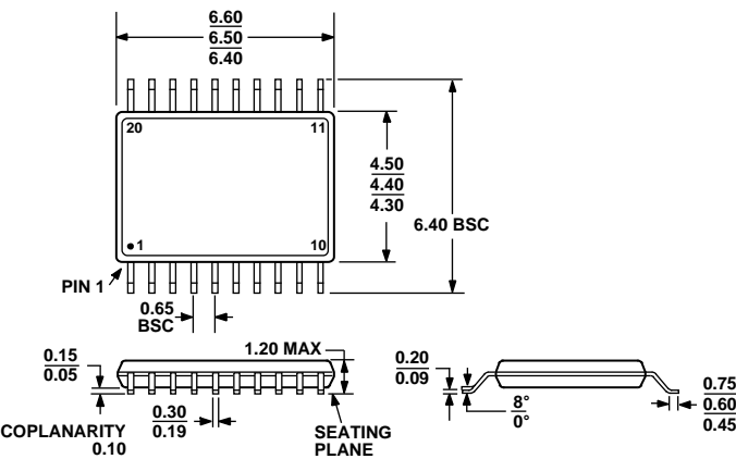
COMPLIANT TO JEDEC STANDARDS MO-153-AC Figure 57. 20-Lead Thin Shrink Small Outline Package [TSSOP] (RU-20) Dimensions show in millimeters
