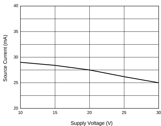
Figure 5. Source Current vs. Supply Voltage
