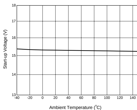
Figure 9. Start-up Voltage vs. Ambient Temperature
