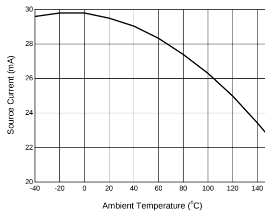
Figure 11. Source Current vs. Ambient Temperature
