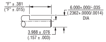
SHAFT TYPE "S" (USES BUSHING R)
