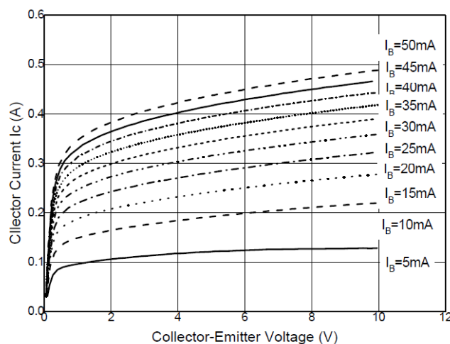
Static Characteristics
