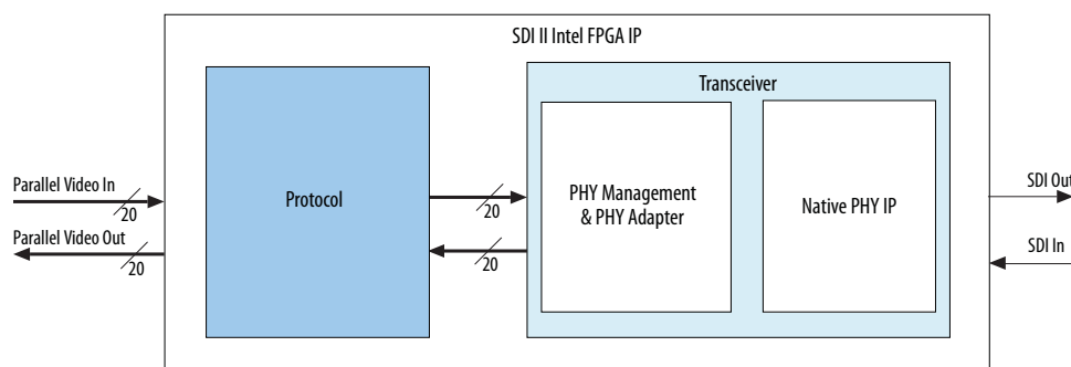
Figure 3. SDI II Intel FPGA IP Core Block Diagram for Arria V, Cyclone V, and Stratix V Devices
