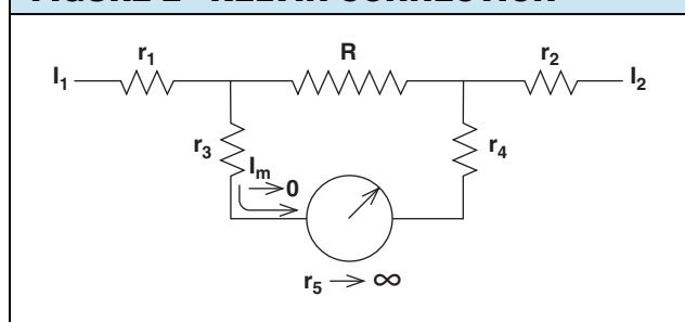
FIGURE 2 - KELVIN CONNECTION
