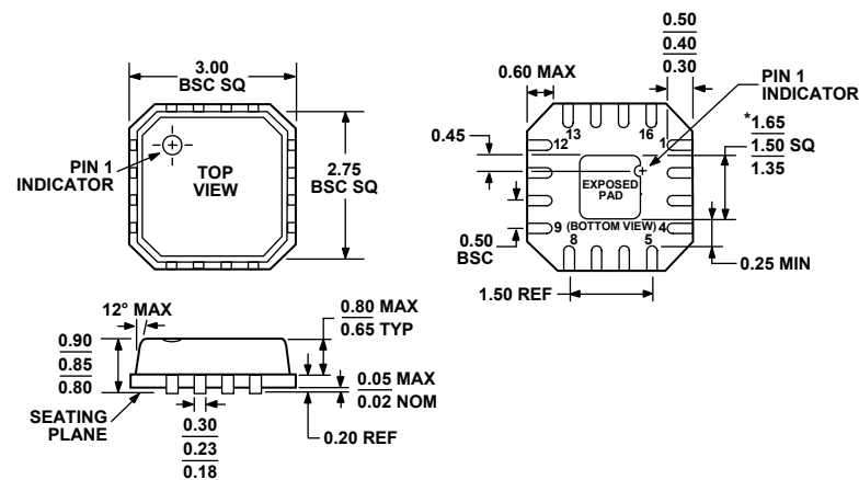
*COMPLIANT TO JEDEC STANDARDS MO-220-VEED-2 EXCEPT FOR EXPOSED PAD DIMENSION. Figure 41. 16-Lead Lead Frame Chip Scale Package [LFCSP_VQ] 3 mm × 3 mm Body, Very Thin Quad (CP-16-3) Dimensions shown in millimeters
