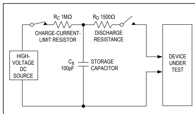
Figure 7a. Human Body ESD Test Model
