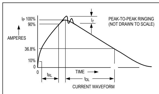
Figure 7b. Human Body Model Current Waveform
