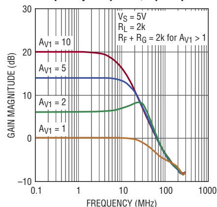
Closed Loop Small Signal Frequency Response, Op Amp 1
