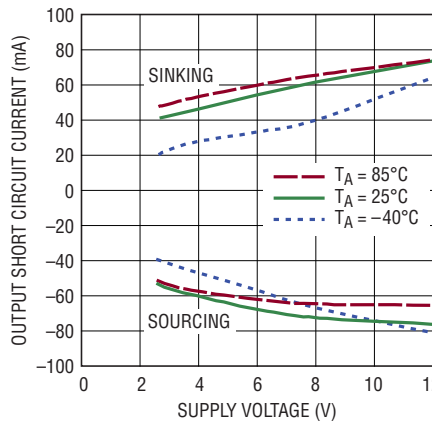
Output Short Circuit Current vs Supply Voltage, Either Output
